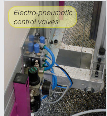
13a 220v power connection. Also requires compressed air
